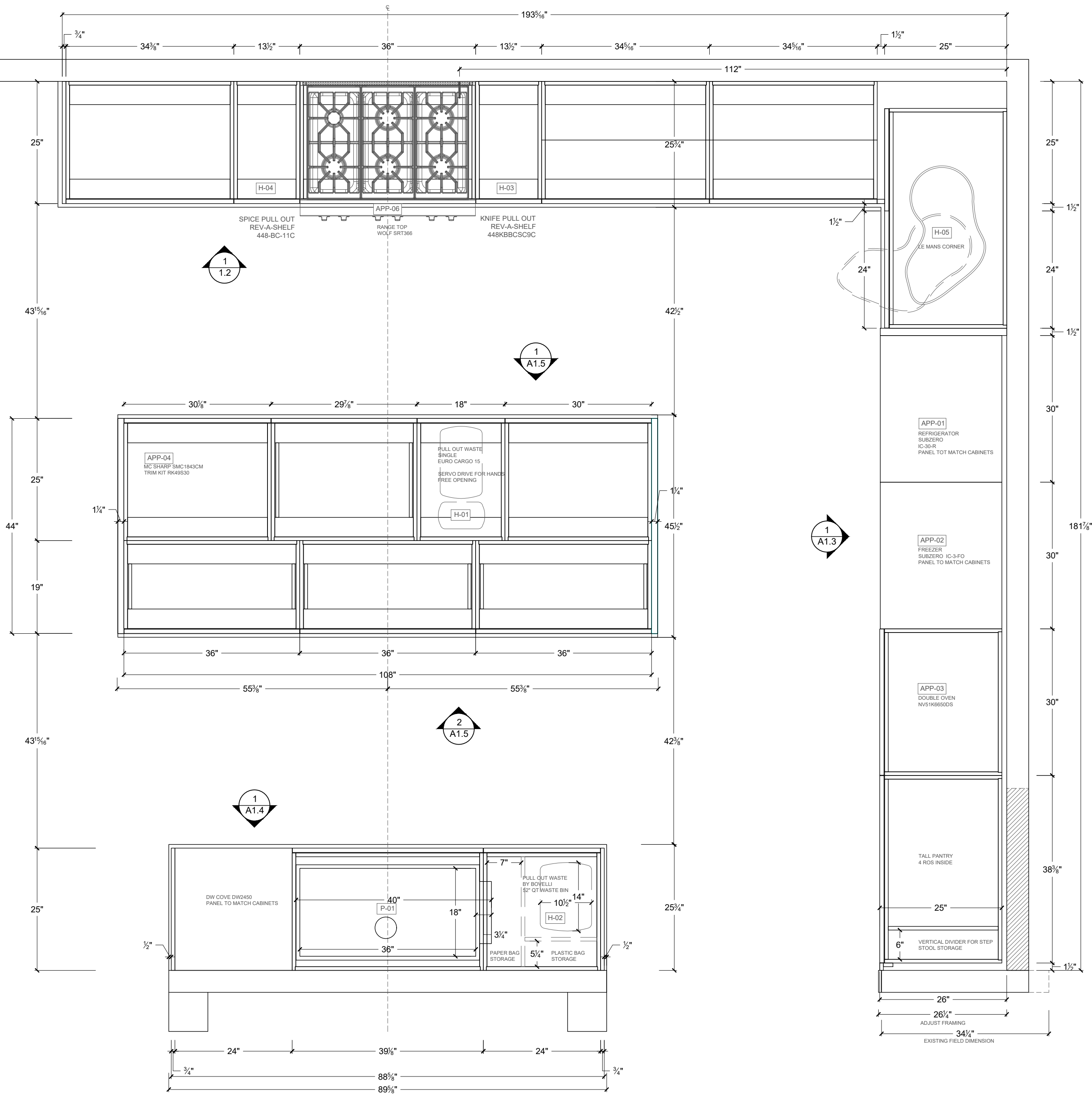
1 PLAN VIEW OF LOEWER CABINETS
